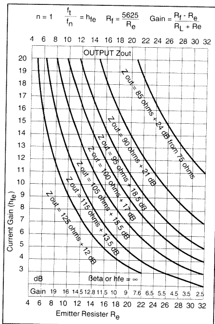
Figure 7. Graph relating beta, gain and output impedance.
