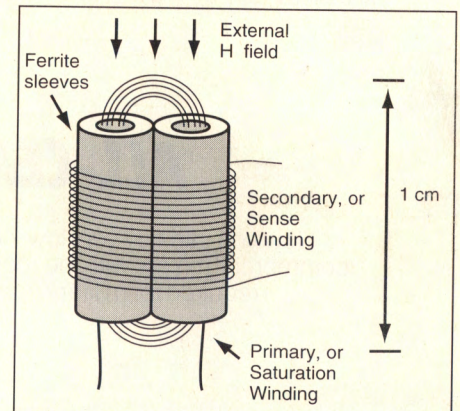
Figure 2. A practical flux-gate magnetometer using two 2673002201 ferrite sleeves and two orthogonal windings.
