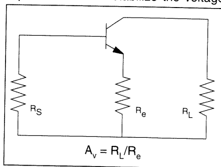
Figure 2. Series feedback circuit showing load, source and emitter resistors.
