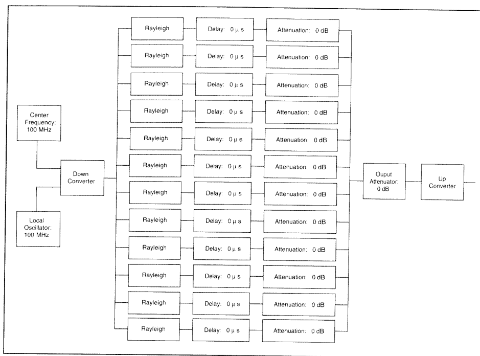
Figure 4. MP-2400 block diagram.
