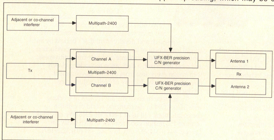
Figure 2. Diversity and interference test using 2 MP-2400s configured for 2 channels with 6 paths each.
