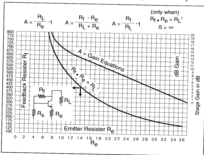
Figure 5. Graph relating R_f , R_e and gain.
