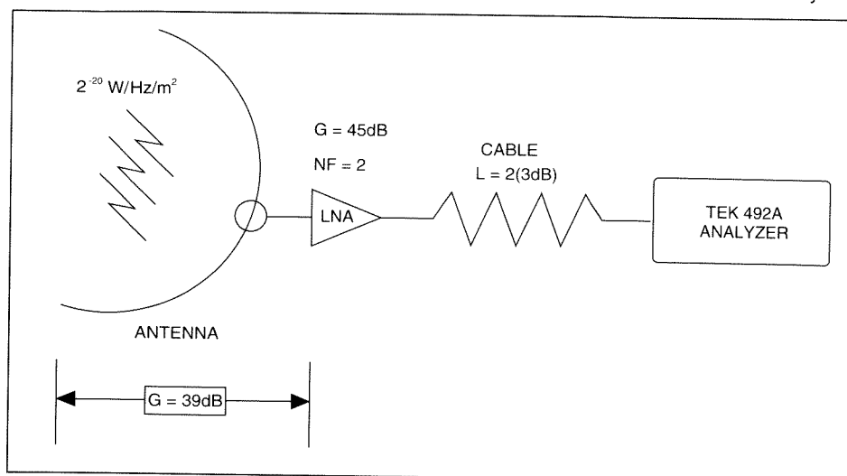
Figure 1. Block diagram of test set-up showing gains, losses and noise figures contributing to the antenna gain measurement.
