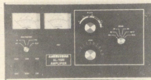
The rugged 3CX1500A7 tube in this HF amplifier delivers over 750 watts of continuous power or up to 4 KW of pulsed output power.
