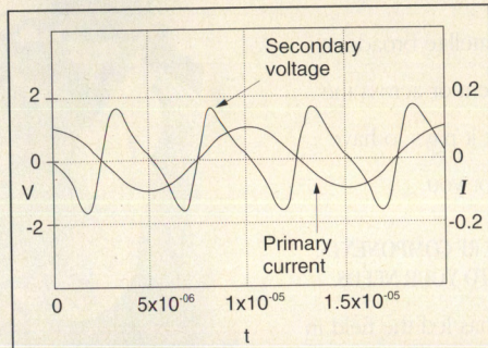
Figure 5. Theoretical detector voltage in 0.5 gauss field showing its second harmonic relationship to primary saturating current.
