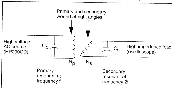
Figure 3. Schematic of flux-gate magnetometer including important resonating capacitors.
