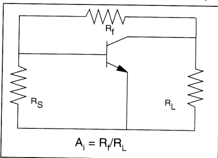
Figure 1. Shunt feedback circuit showing load, source and feedback resistors.
