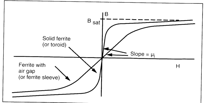
Figure 4. Simplified B-H curves for toroid and sleeve of the same ferrite material.
