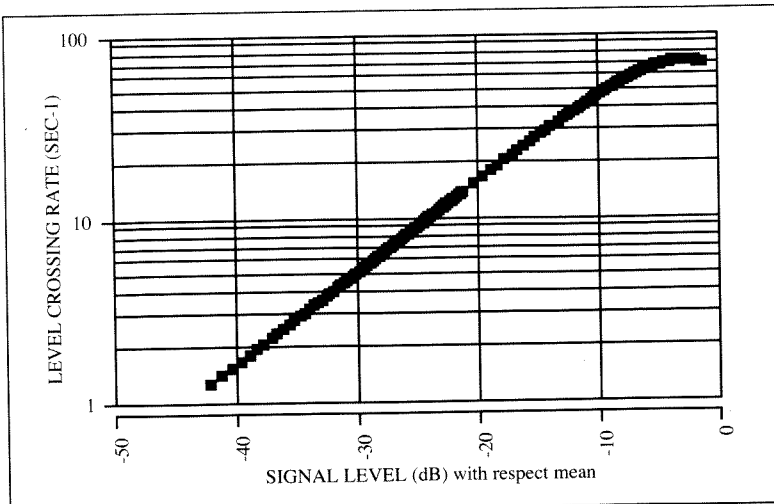
Figure 4. Level crossing rate.
