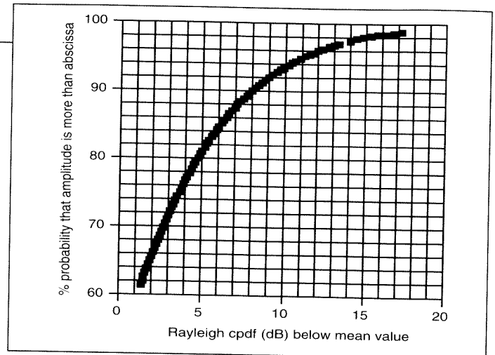
Figure 3. Rayleigh Cumulative Distribution Function.
