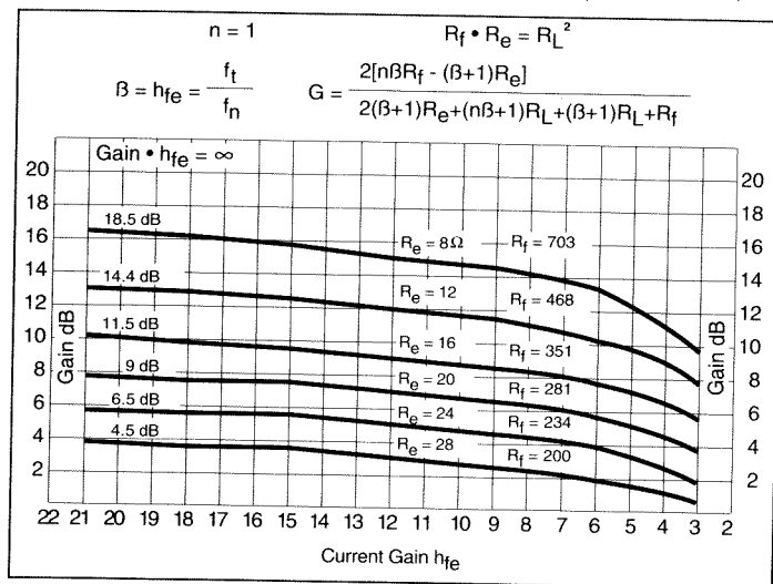
Figure 4. Gain versus different betas.
