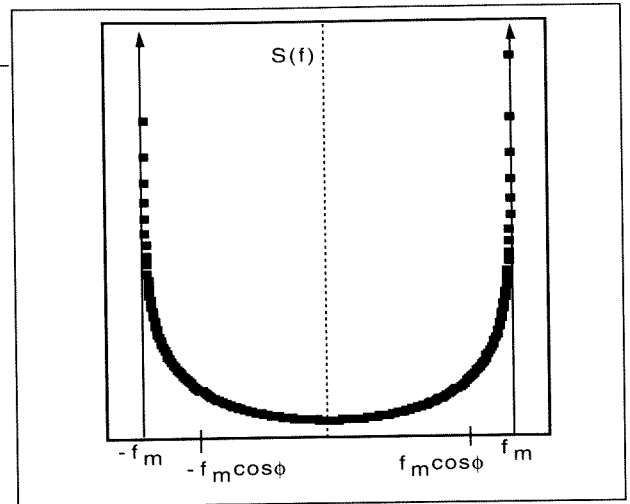
Figure 5. Rayleigh power spectra.
