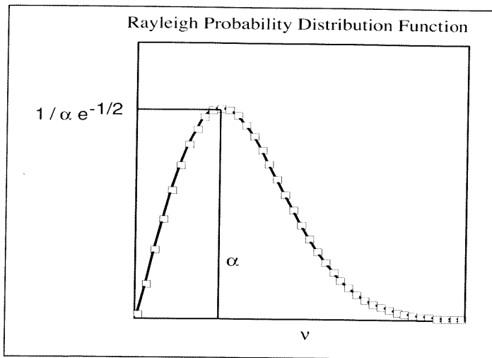
Figure 2. Rayleigh Probability Distribution Function.
