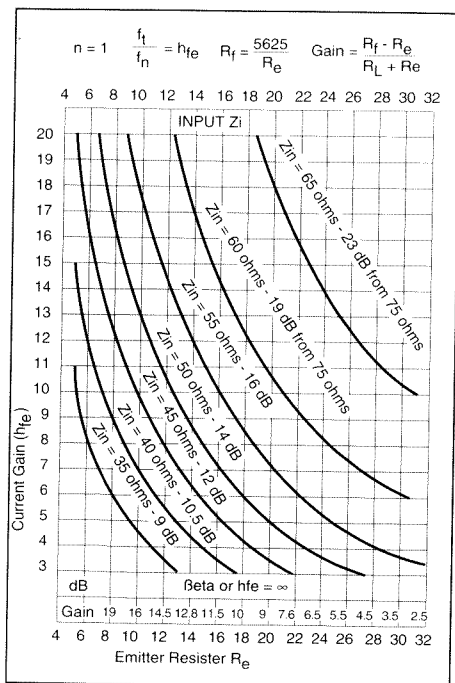
Figure 6. Graph relating beta, gain and input impedance.
