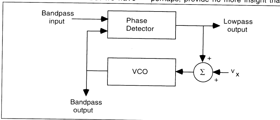
Figure 4. Block diagram of a PLL with an external applied voltage, v_x .
