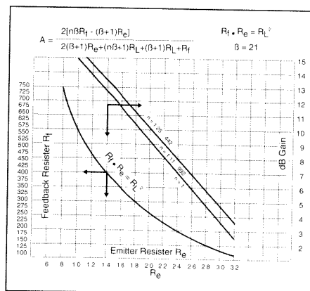
Figure 10. Gain versus beta in high frequency operation and with variable n .
