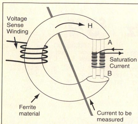
Figure 1. Simplified magnetic flux gate for measuring DC current.
