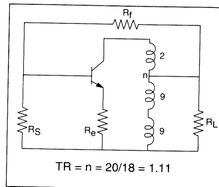
Figure 3. Double feedback circuit.
