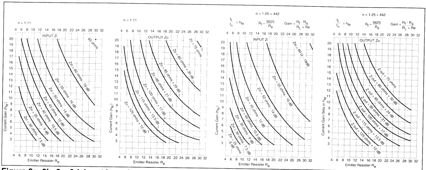
Figure 9a, 9b, 9c, 9d. Input impedances (9a, 9c) and output impedances (9b, 9d) for n = 1.11 (9a, 9b) and for n = 1.25 (9c, 9d).
