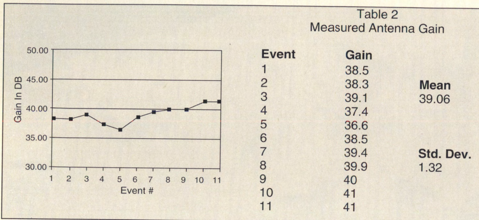
Figure 3. Test results of 11 antennas using the solar source measurement technique.
