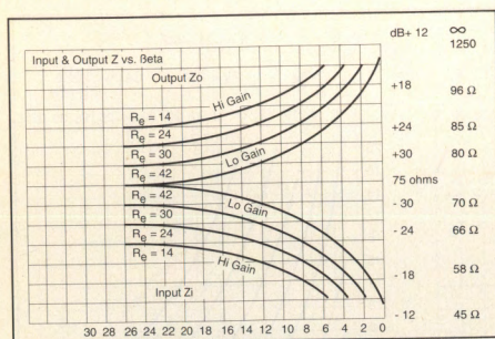
Figure 8. Graph showing how input and output impedances vary with beta.
