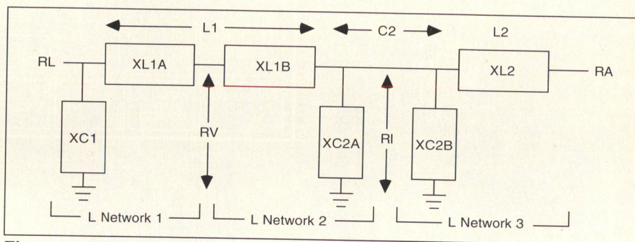
Figure 1. Equivalent schematic of the PI-L output network.
