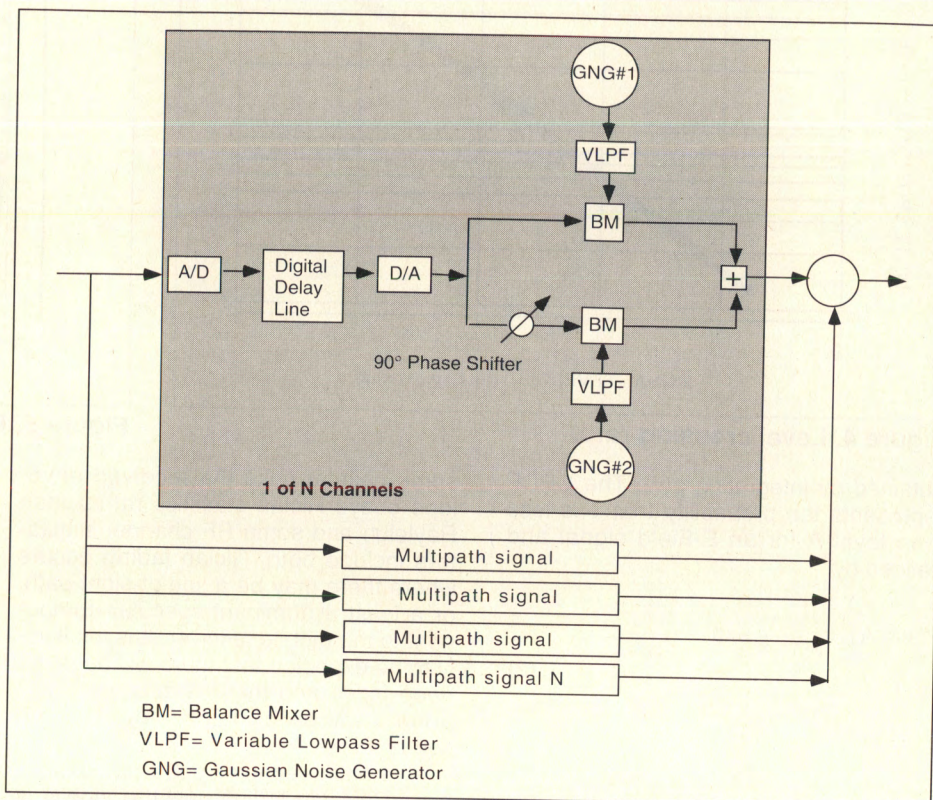
Figure 6. Rayleigh RF channel simulator hardware.
